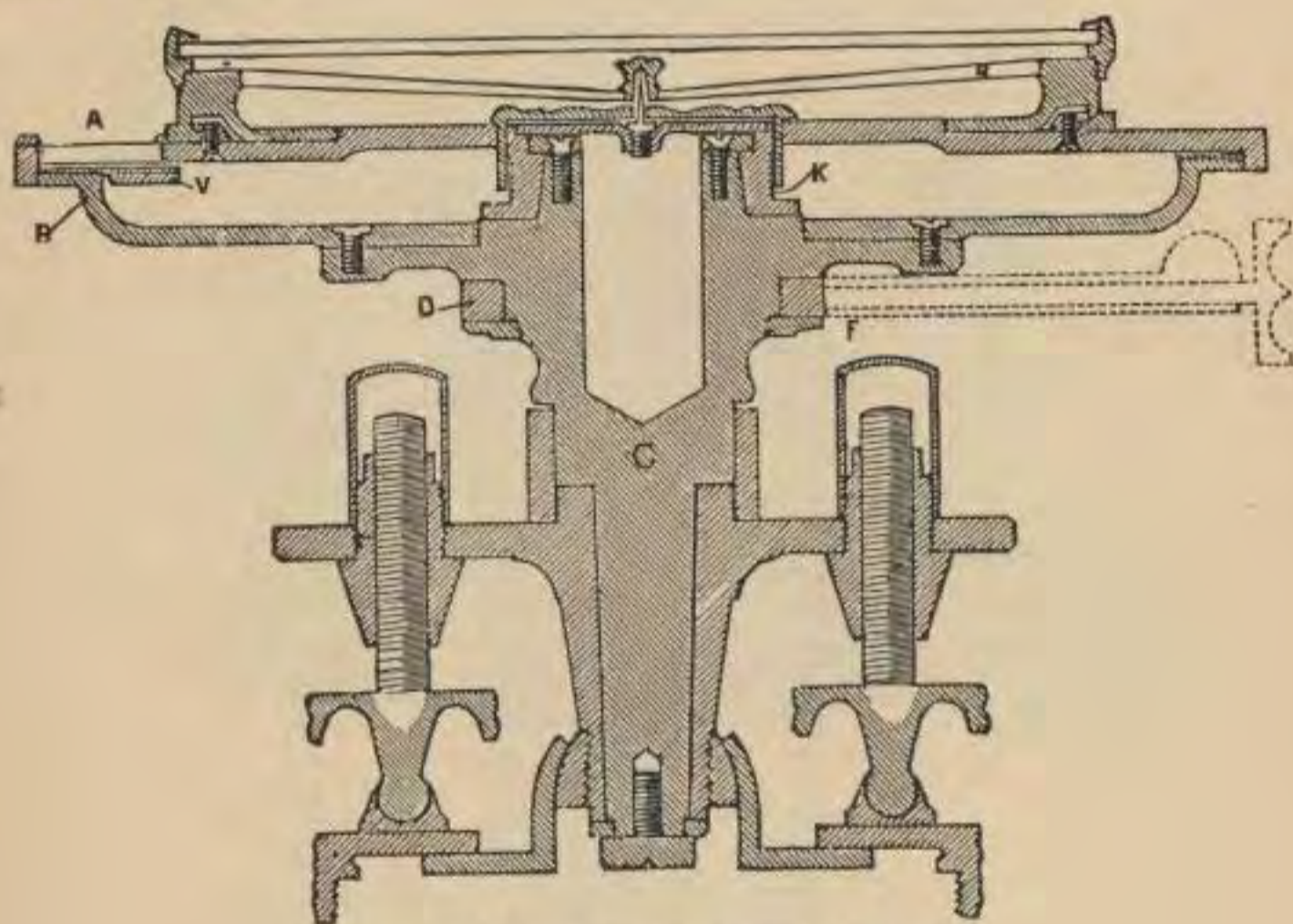
THE SOCKETS AND CIRCULAR PLATES.
