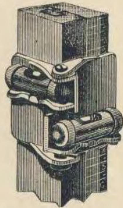
ROD-LEVEL AS APPLIED TO A ROD.
