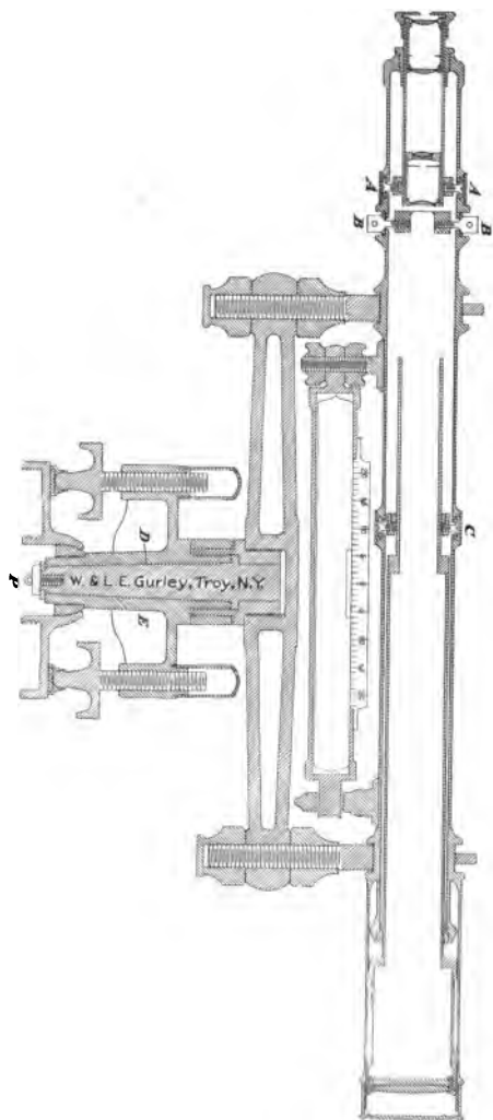
SECTIONAL VIEW OF Y LEVEL
