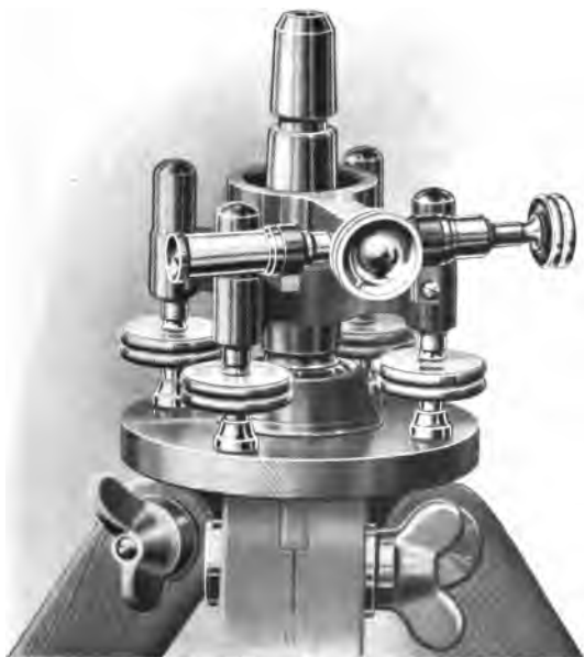
Nos. 176 and 242 LEVELING HEAD
