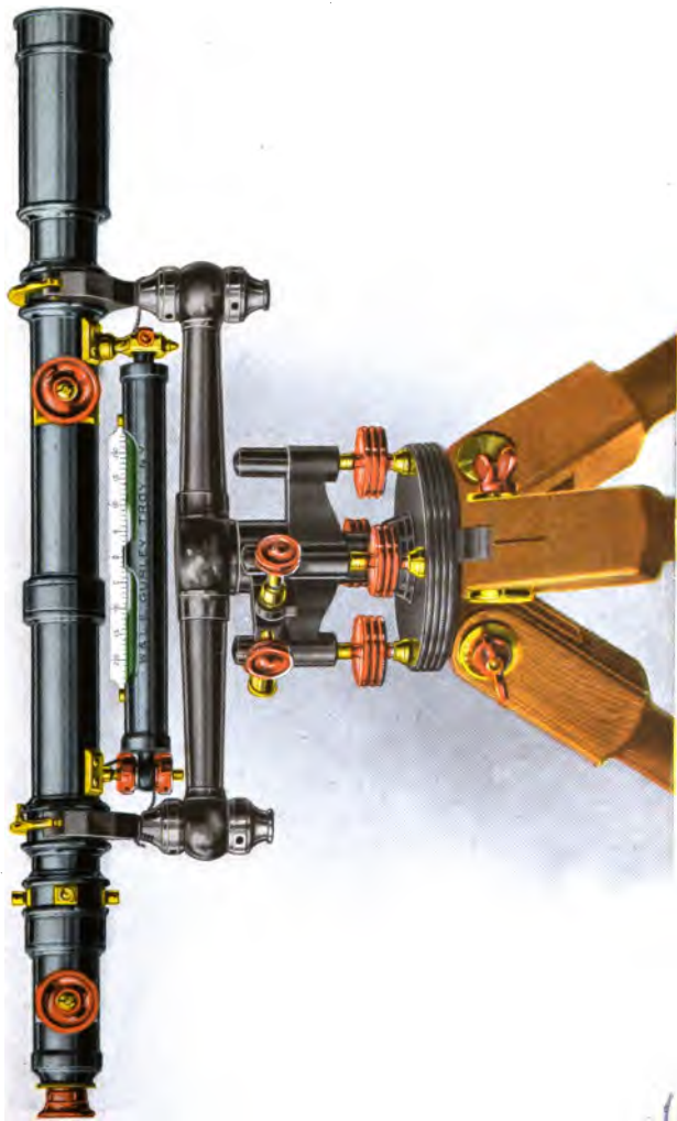
No. 376 20 INCH Y LEVEL [Page 195]
