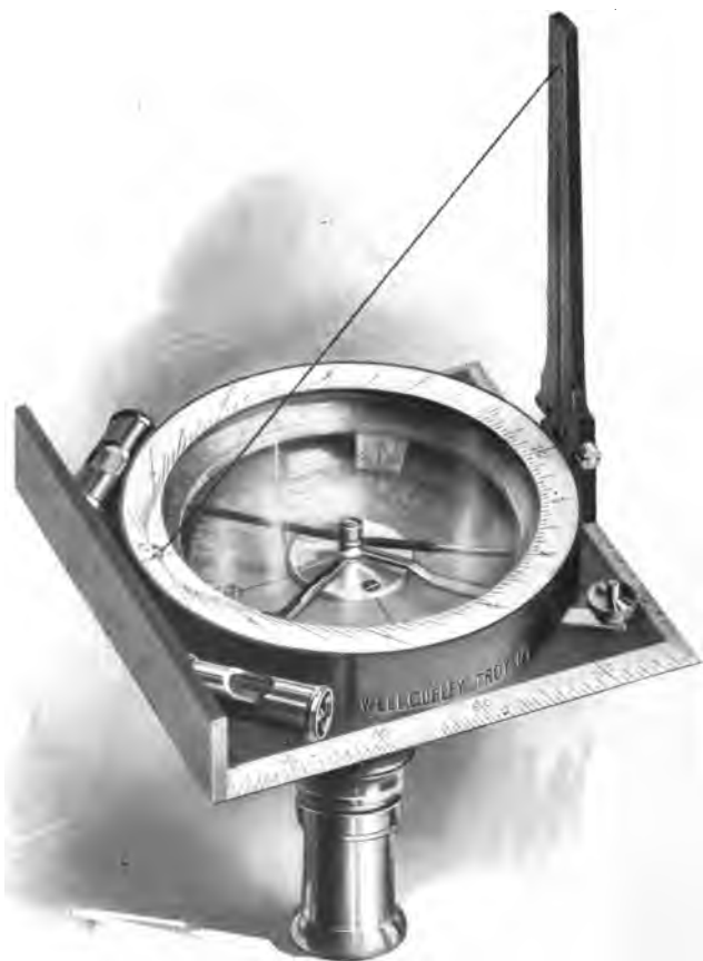
No. 348 BRASS DIAL COMPASS
