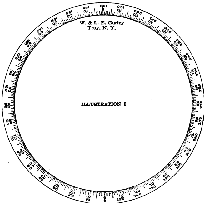
ILLUSTRATION I — The figures are in two rows, the outer from 0 to 360, and the inner in quadrants from 0 to 90. This is the customary form.
