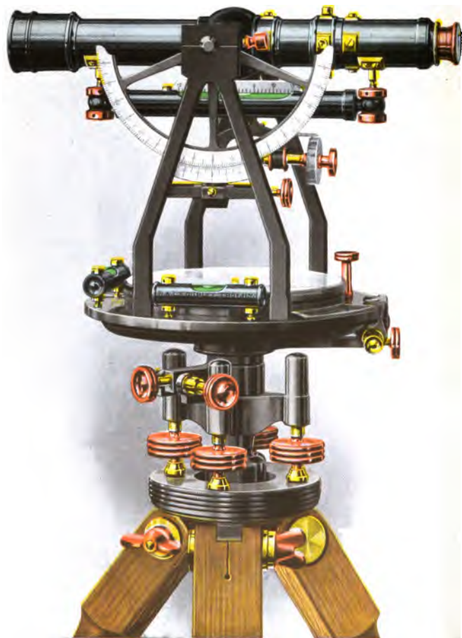
No. 16 ENGINEERS TRANSIT, TWO VERNIERS TO LIMB [Page 44]
