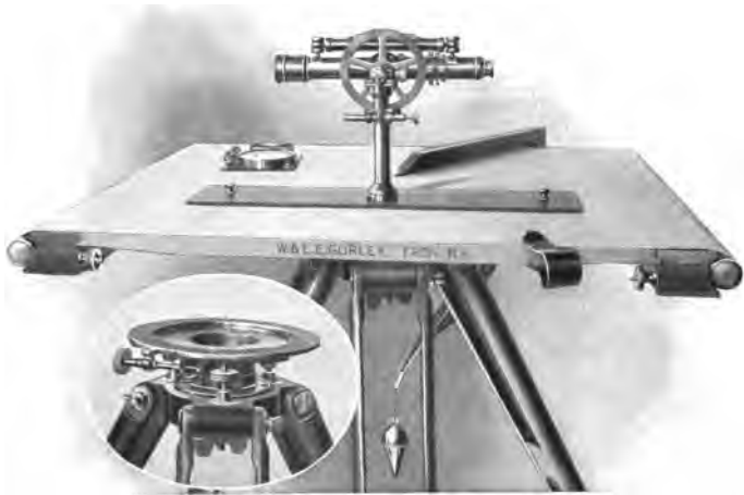
No. 549. PLANE TABLE OUTFIT
