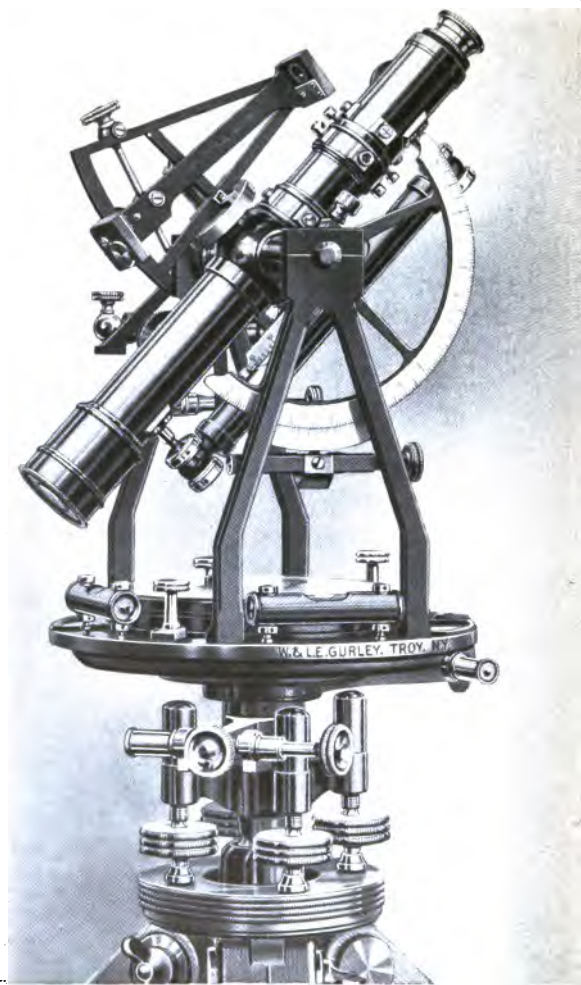
No. 17 ENGINEERS TRANSIT, WITH SOLAR ATTACHMENT, TWO VERNIERS TO LIMB [Page 46]
