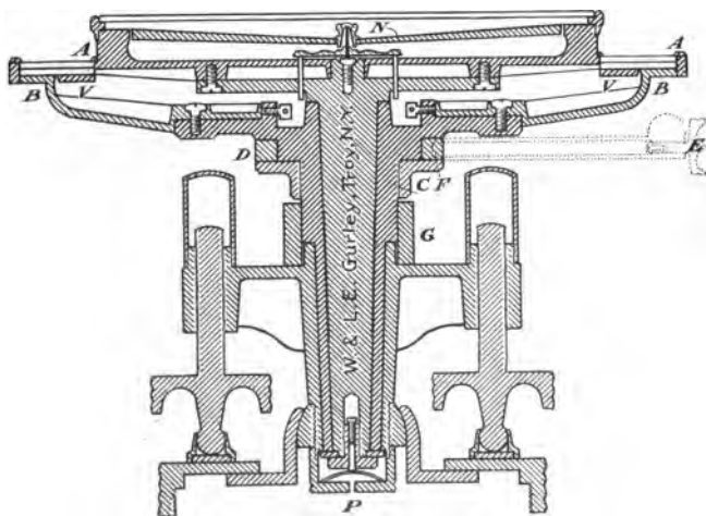
SOCKETS AND CIRCULAR PLATES
