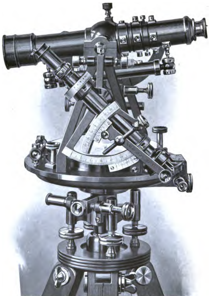
No. 32 TELESCOPIC SOLAR
