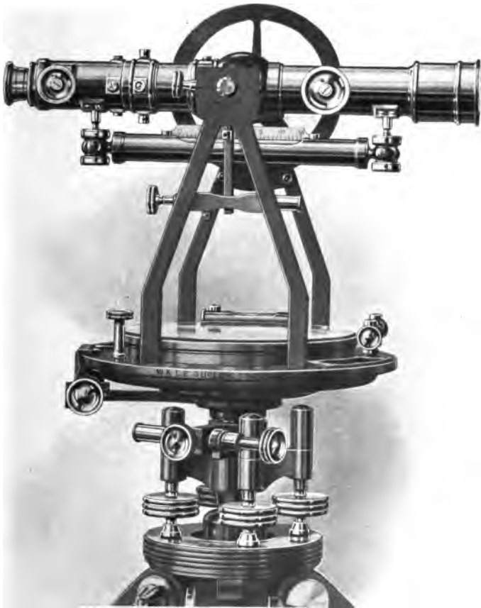
No. 14 ENGINEERS TRANSIT, TWO VERNIERS TO LIMB
