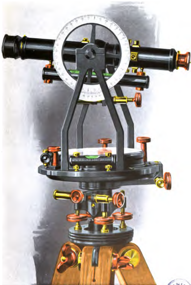
No. 100 RECONNOISSANCE TRANSIT, ONE VERNIER TO LIMB [Page 69]
